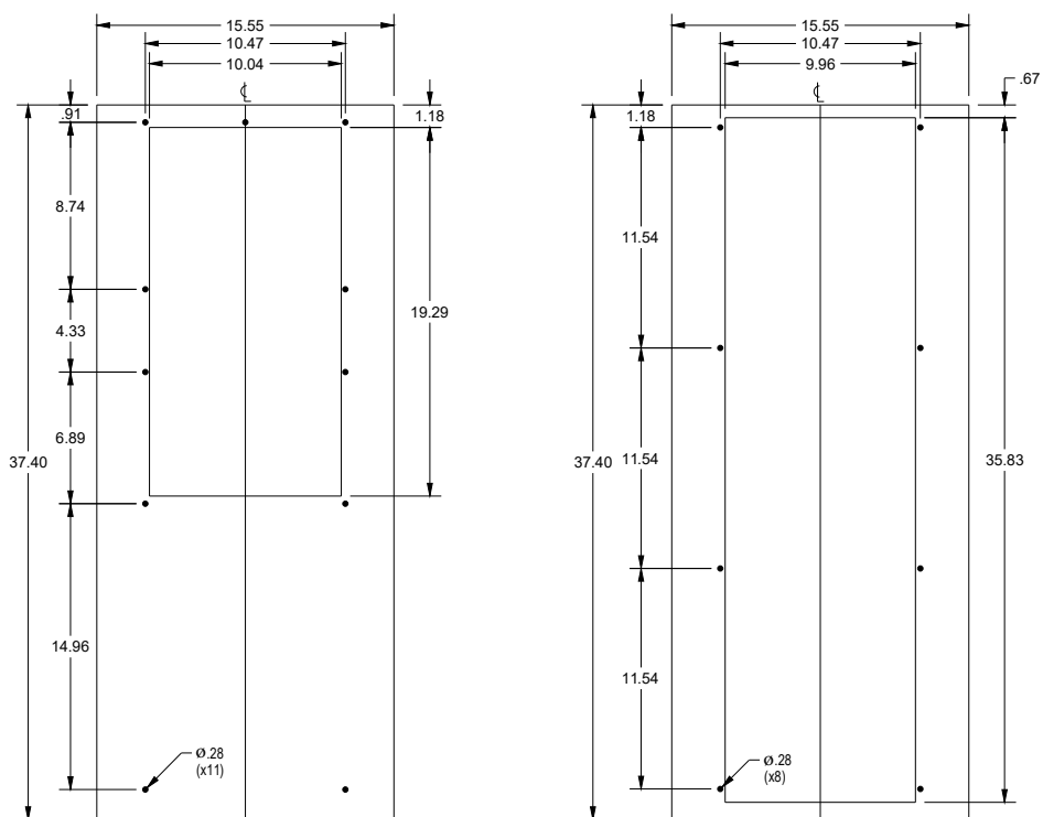
CUTOUT FOR INTERNAL INSTALLATION
