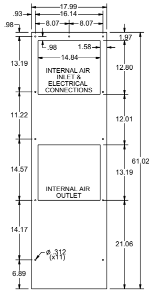
MOUNTING PATTERN
